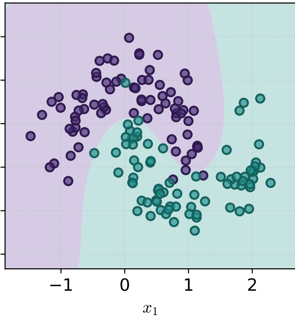
(b) \gamma = 1 : acc. test = 0.98
