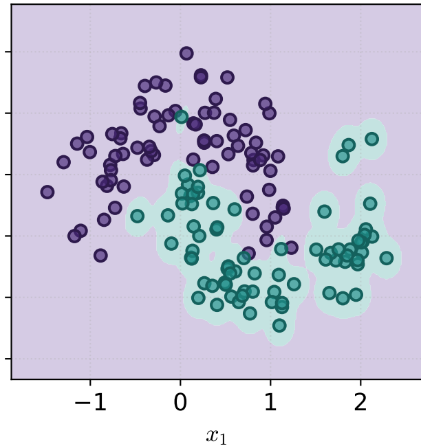
(c) \gamma = 100 : acc. test = 0.80
