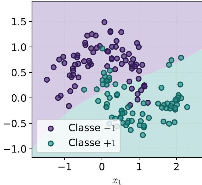
(a) \gamma = 0.1 : acc. test = 0.90
